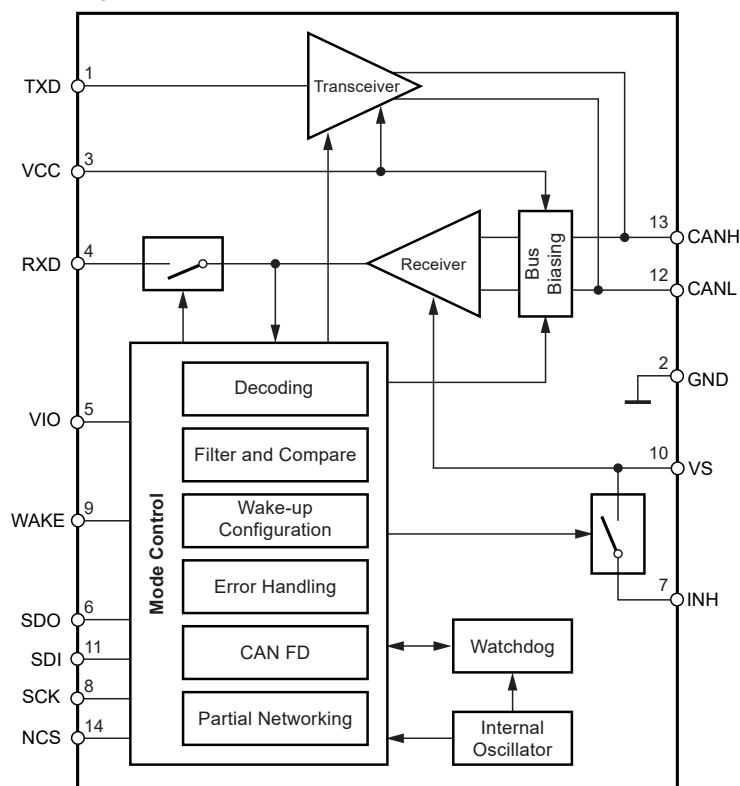
Figure 1. Simplified Block Diagram
