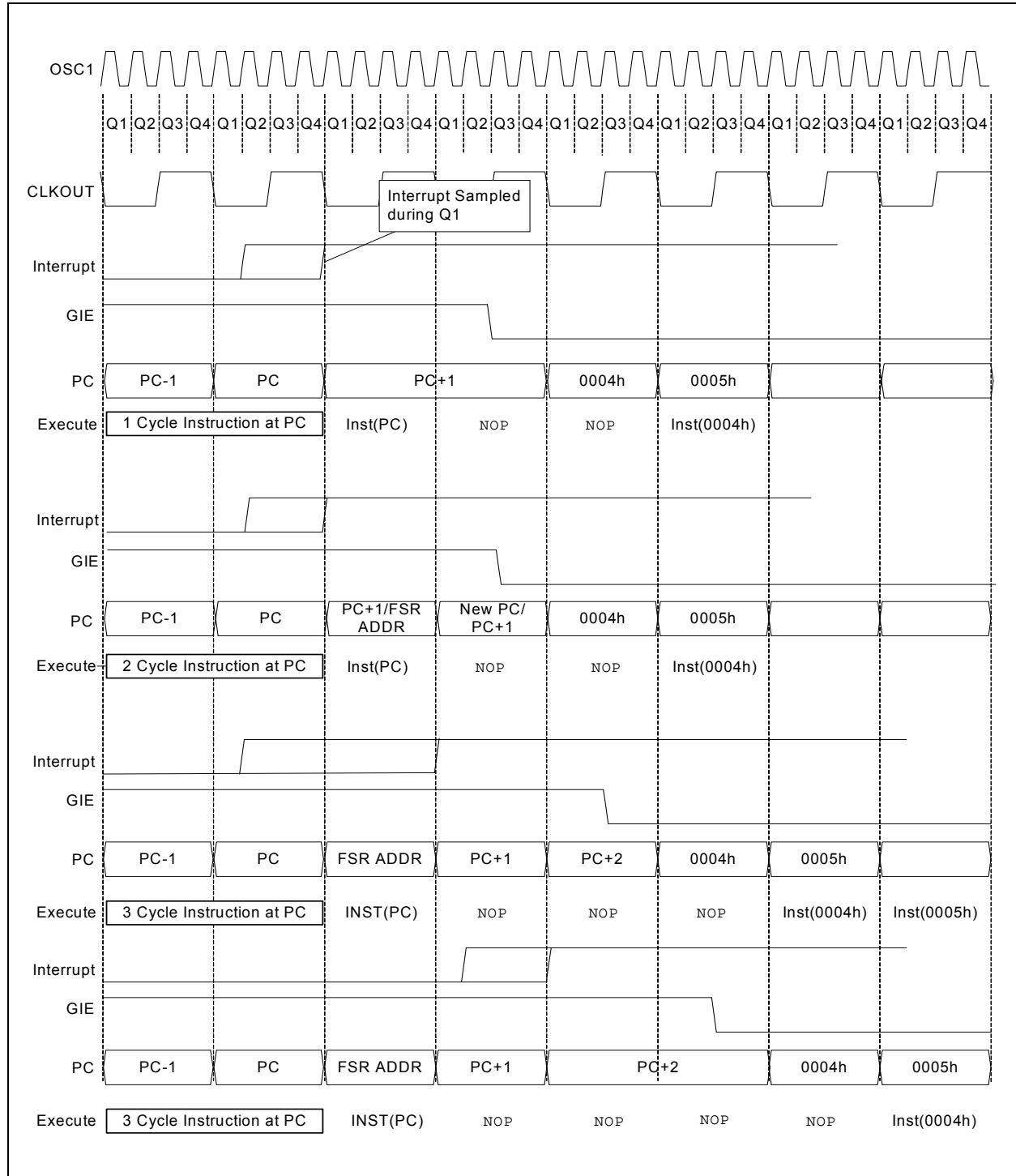
FIGURE 7-2: INTERRUPT LATENCY
