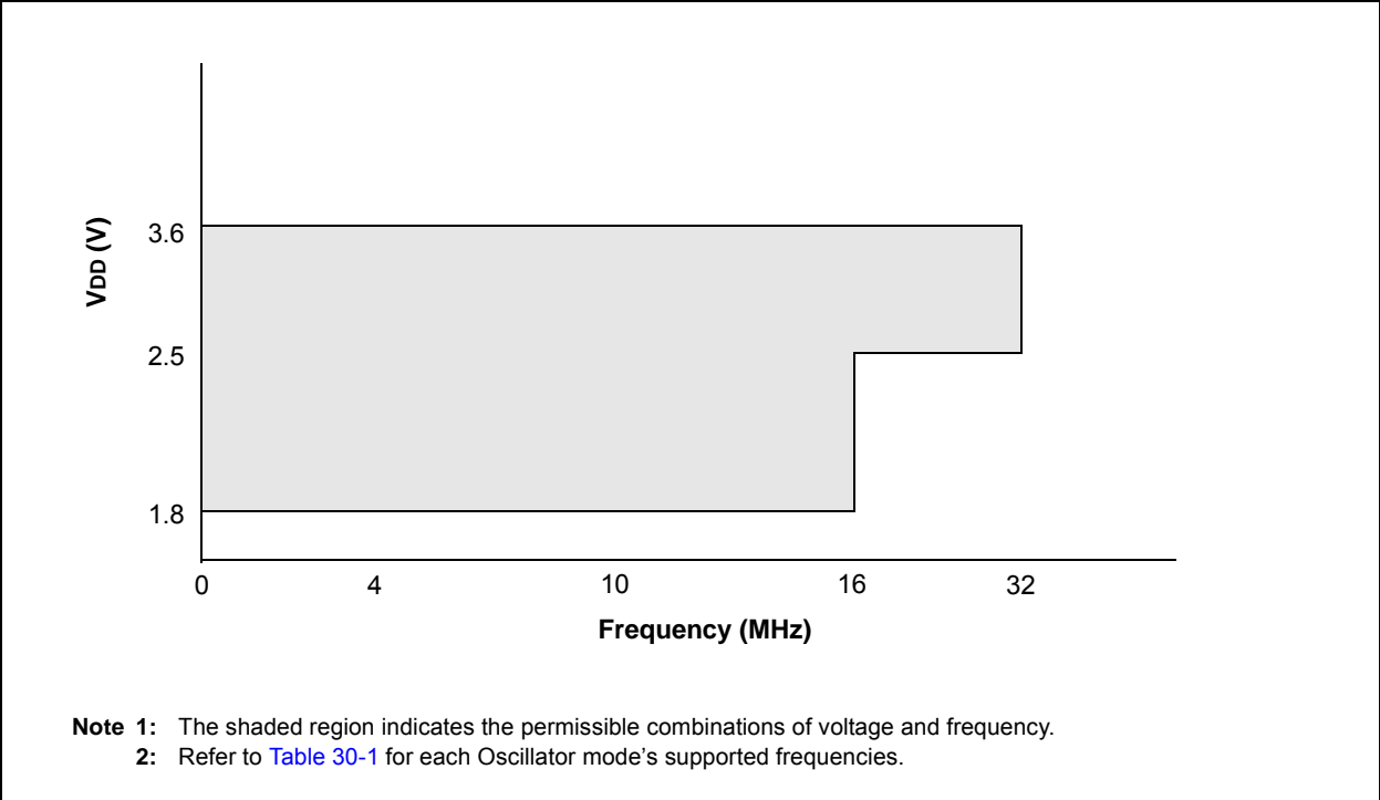
FIGURE 30-2: PIC16LF1946/47 VOLTAGE FREQUENCY GRAPH, -40°C ≤ TA ≤ +125°C
