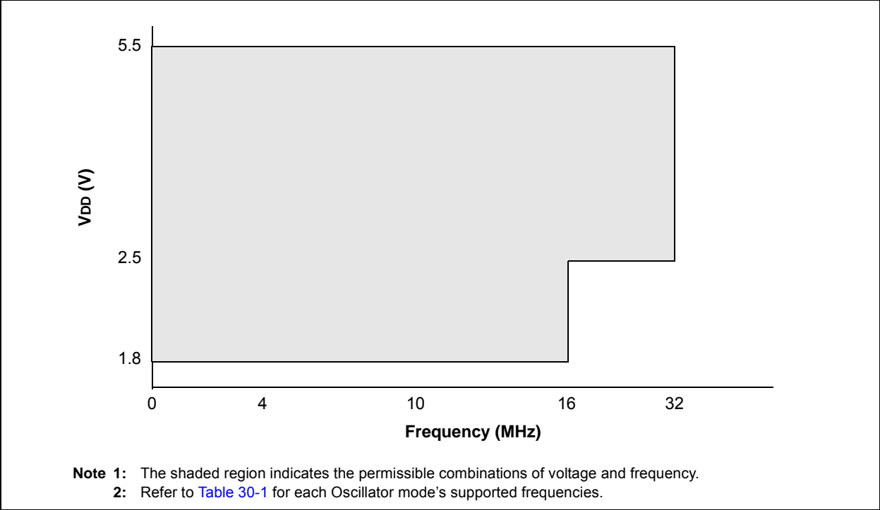
FIGURE 30-1: PIC16F1946/47 VOLTAGE FREQUENCY GRAPH, -40°C ≤ TA ≤ +125°C
