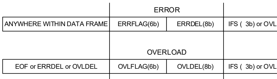
Figure 38-12. Error and Overload Frame
